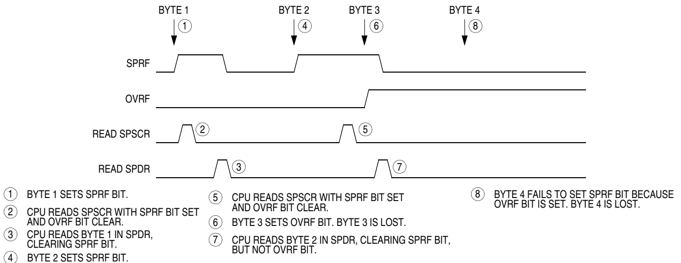
Figure 16-8. Missed Read of Overflow Condition
