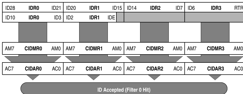
Figure 11-4. Single 32-Bit Maskable Identifier Acceptance Filter
