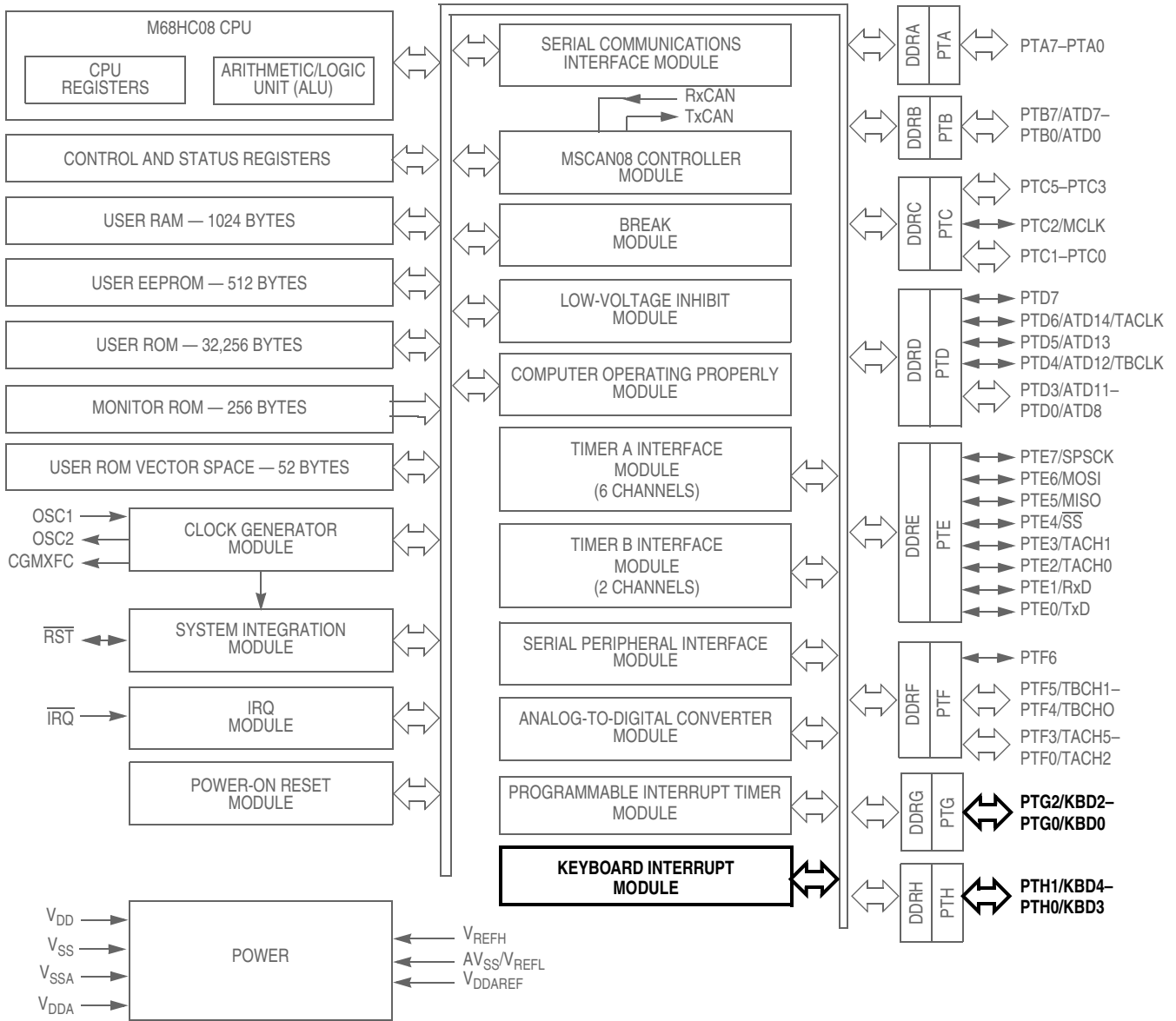
Figure 8-1. Block Diagram Highlighting KBD Block and Pins
