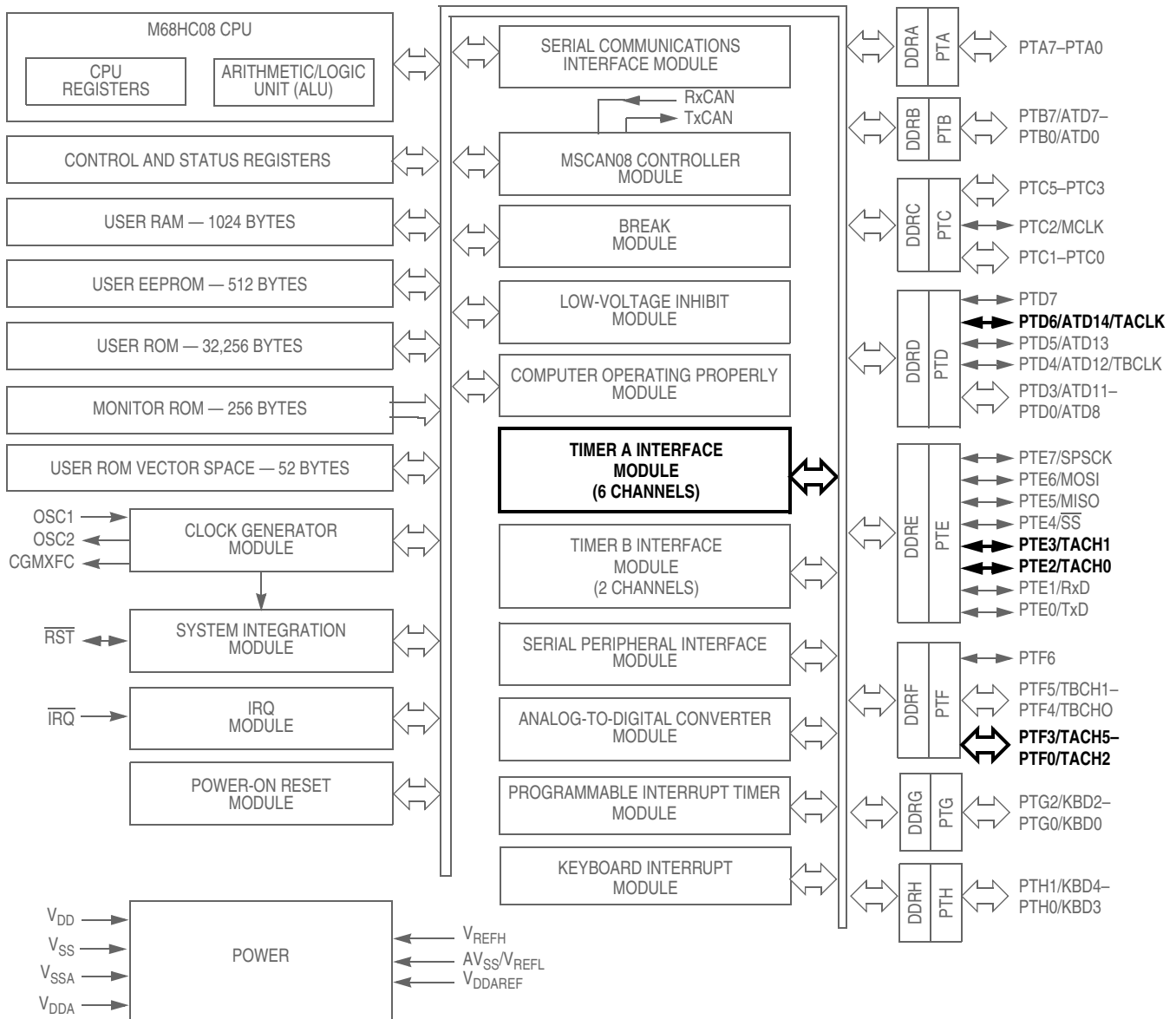
Figure 17-1. Block Diagram Highlighting TIMA Block and Pins
