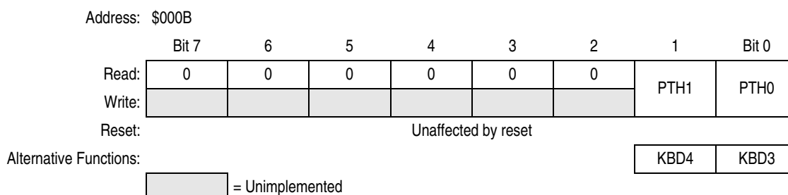
Figure 13-23. Port H Data Register (PTH)
