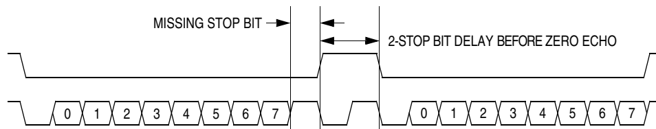
Figure 19-10. Break Transaction
