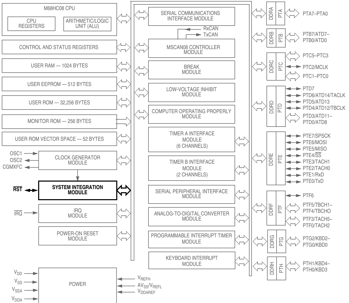
Figure 15-1. Block Diagram Highlighting SIM Block and Pin
