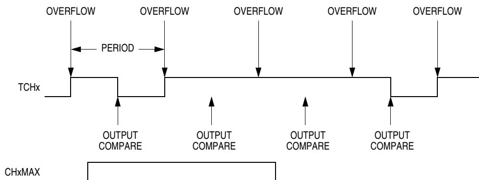
Figure 17-9. CHxMAX Latency
