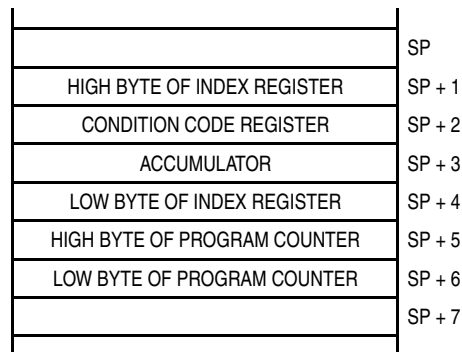
Figure 19-13. Stack Pointer at Monitor Mode Entry
