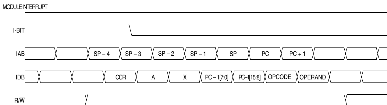
Figure 15-10. Interrupt Recovery
