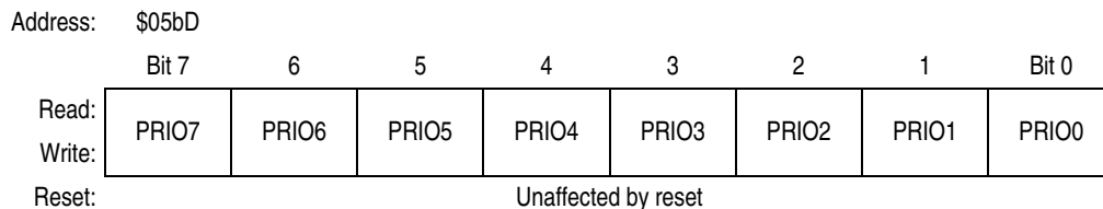
Figure 11-14. Transmit Buffer Priority Register (TBPR)
