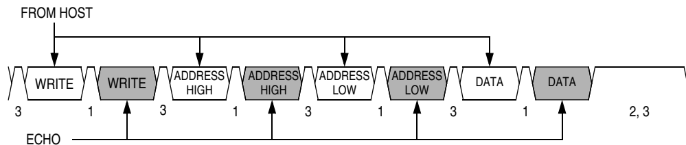
Figure 19-11. Read Transaction
