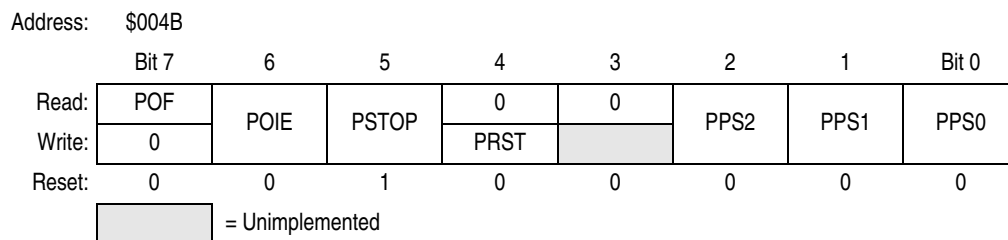
Figure 12-4. PIT Status and Control Register (PSC)
