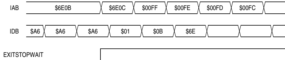
Figure 15-13. Wait Recovery from Interrupt
