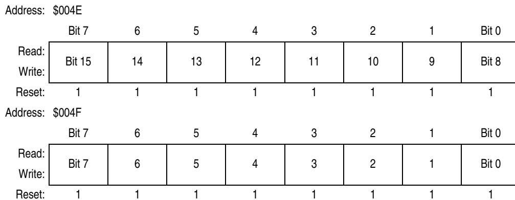
Figure 12-6. PIT Counter Modulo Registers (PMDH–PMDL)
