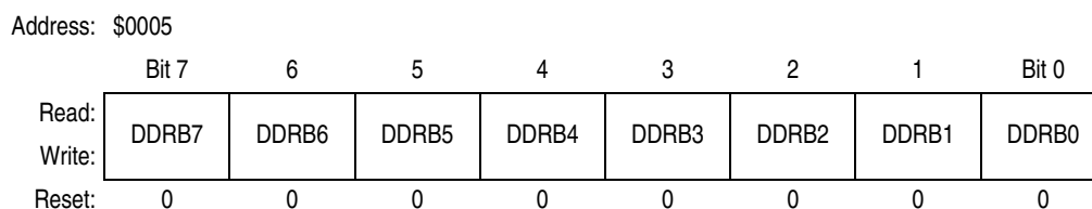
Figure 13-6. Data Direction Register B (DDRB)
