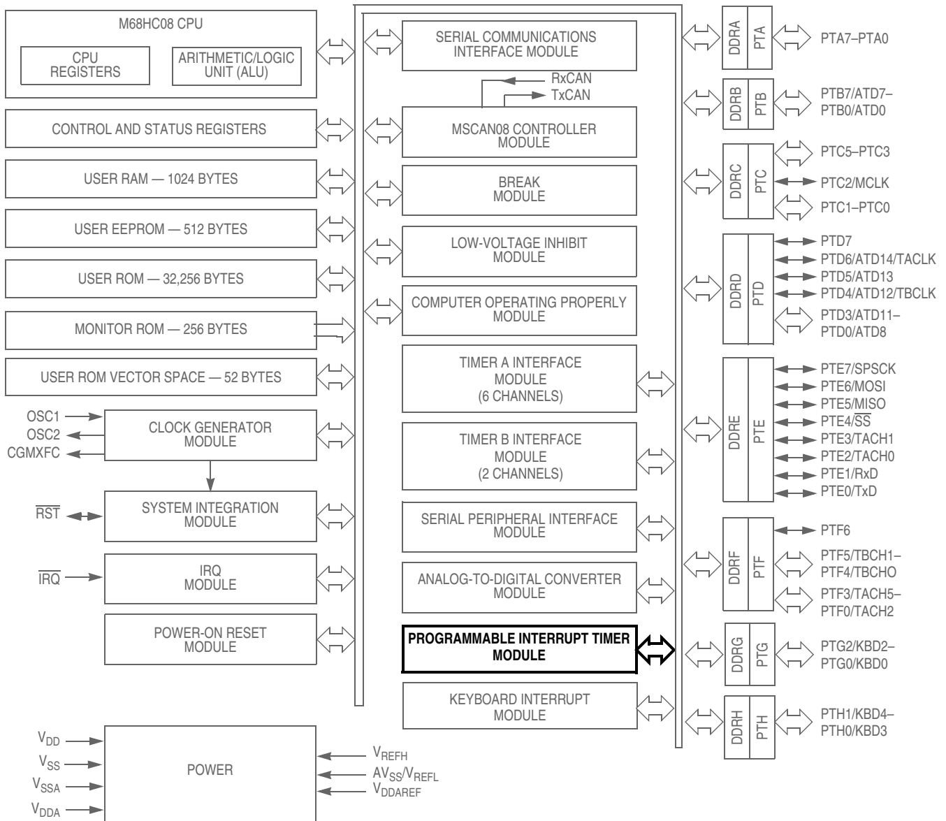
Figure 12-2. Block Diagram Highlighting PIT Block
