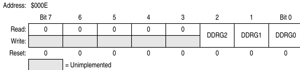
Figure 13-21. Data Direction Register G (DDRG)
