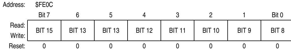
Figure 19-5. Break Address Register (BRKH)
