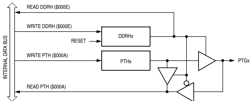
Figure 13-25. Port H I/O Circuit
