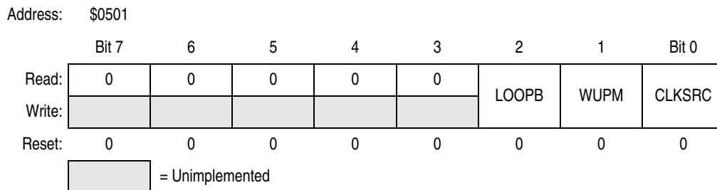
Figure 11-17. Module Control Register (CMCR1)
