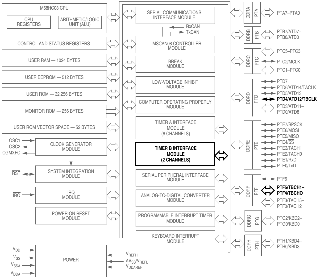
Figure 18-1. Block Diagram Highlighting TIMB Block and Pins
