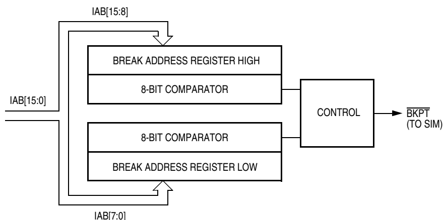
Figure 19-2. Break Module Block Diagram
