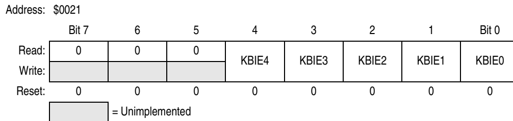
Figure 8-5. Keyboard Interrupt Enable Register (KBIER)
