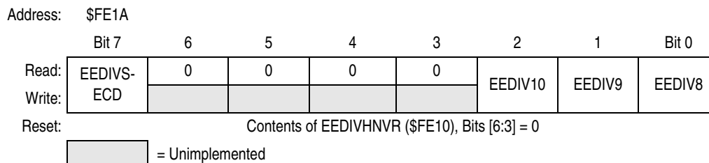
Figure 2-7. EEDIV Divider High Register (EEDIVH)
