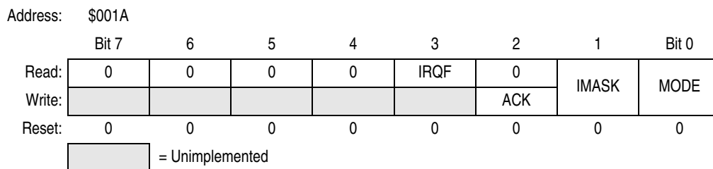
Figure 7-5. IRQ Status and Control Register (ISCR)
