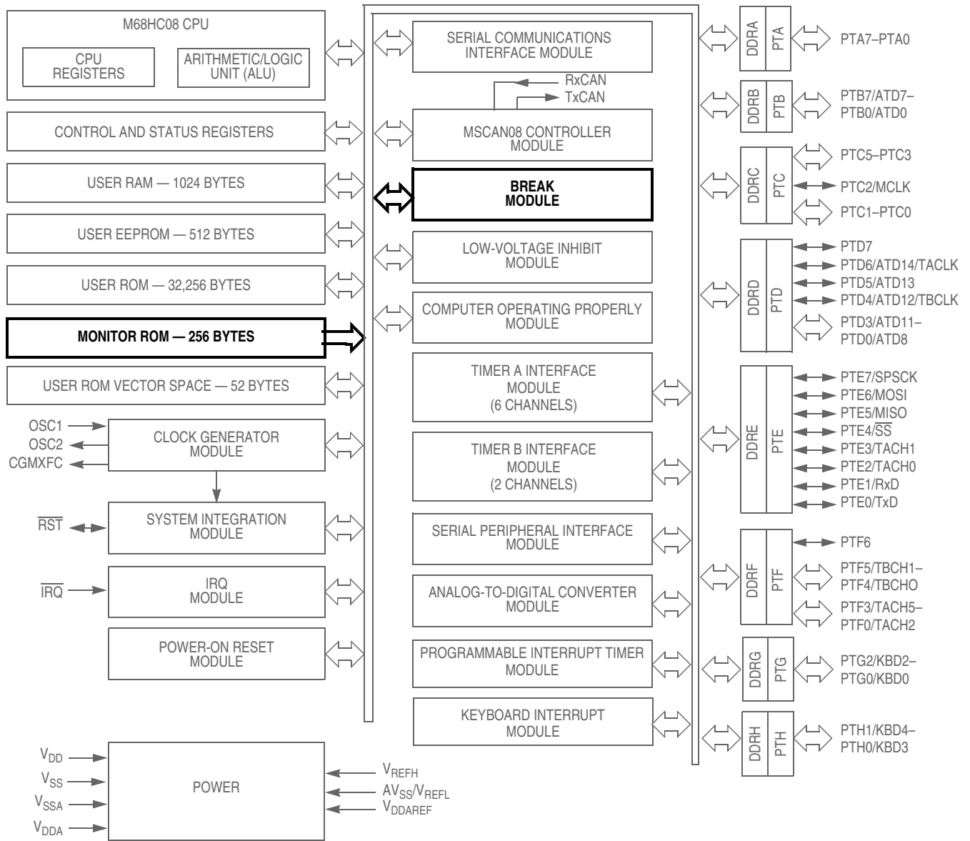
Figure 19-1. Block Diagram Highlighting BRK and MON Blocks
