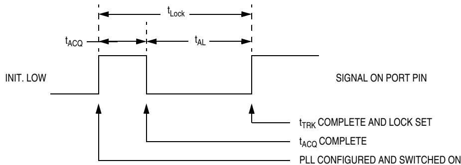
Figure 4-7. Typical Lock Time Waveform Example
