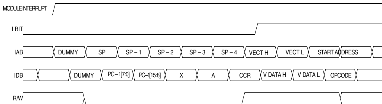
Figure 15-9. Interrupt Entry
