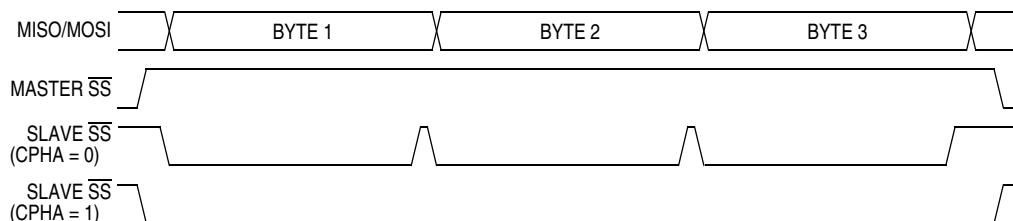
Figure 16-12. CPHA/ \overline{SS} Timing
