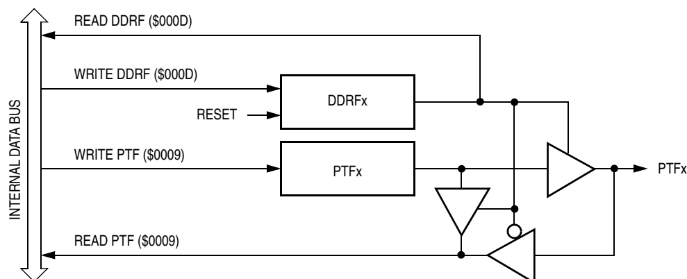
Figure 13-19. Port F I/O Circuit
