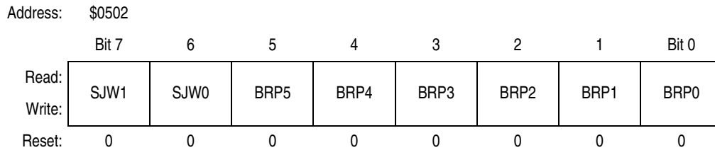
Figure 11-18. Bus Timing Register 0 (CBTR0)
