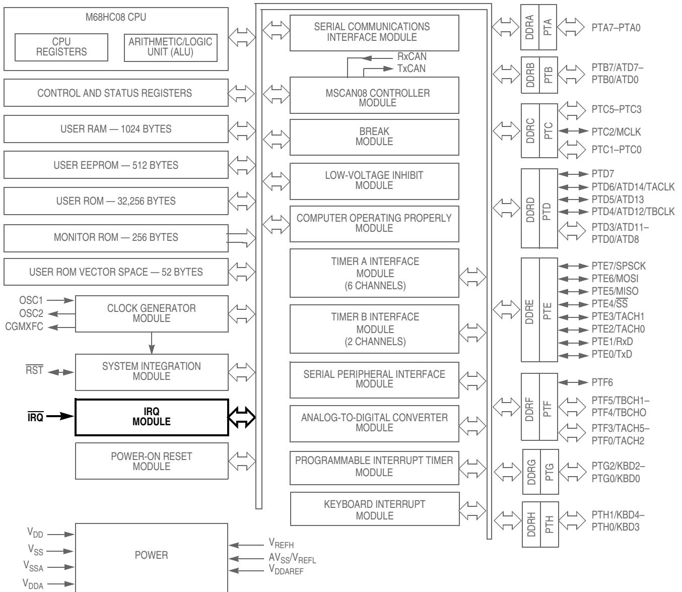
Figure 7-2. Block Diagram Highlighting IRQ Block and Pins
